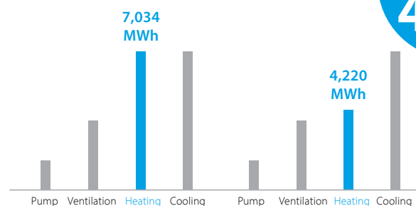
Heat recovery - before vs 1 year after retrofitting - Italian TV station - 40% energy saving
