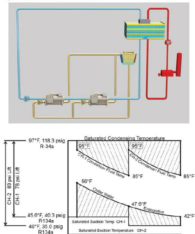
Figure 8: Series Parallel Flow
