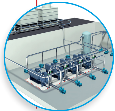
CHILLER OR AHU PLANT
