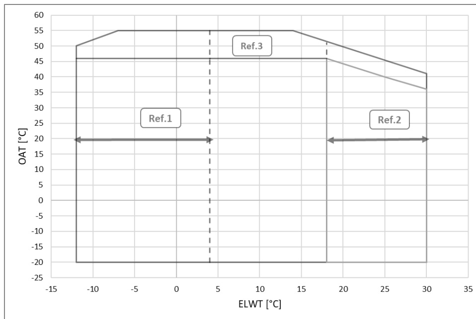
Fig. 5 – EWAH-TZD envelope Silver
