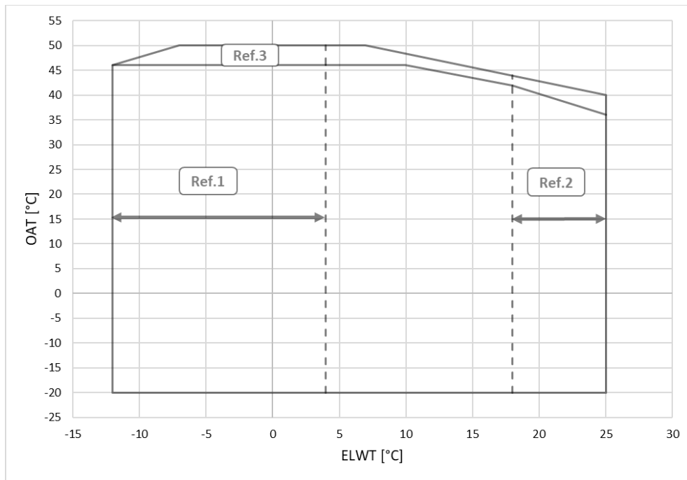
Fig. 8 – EWAD-TZD envelope Silver
