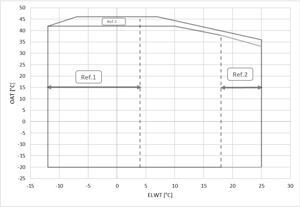
Fig. 11 – EWAS-TZD envelope Silver
