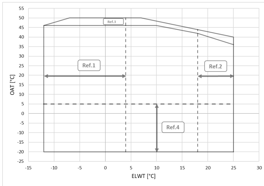
Fig. 8 – EWAD-TZD envelope Silver
