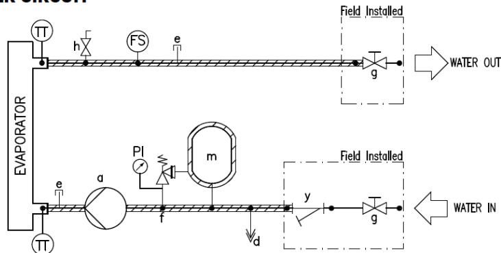
WATER CIRCUIT
